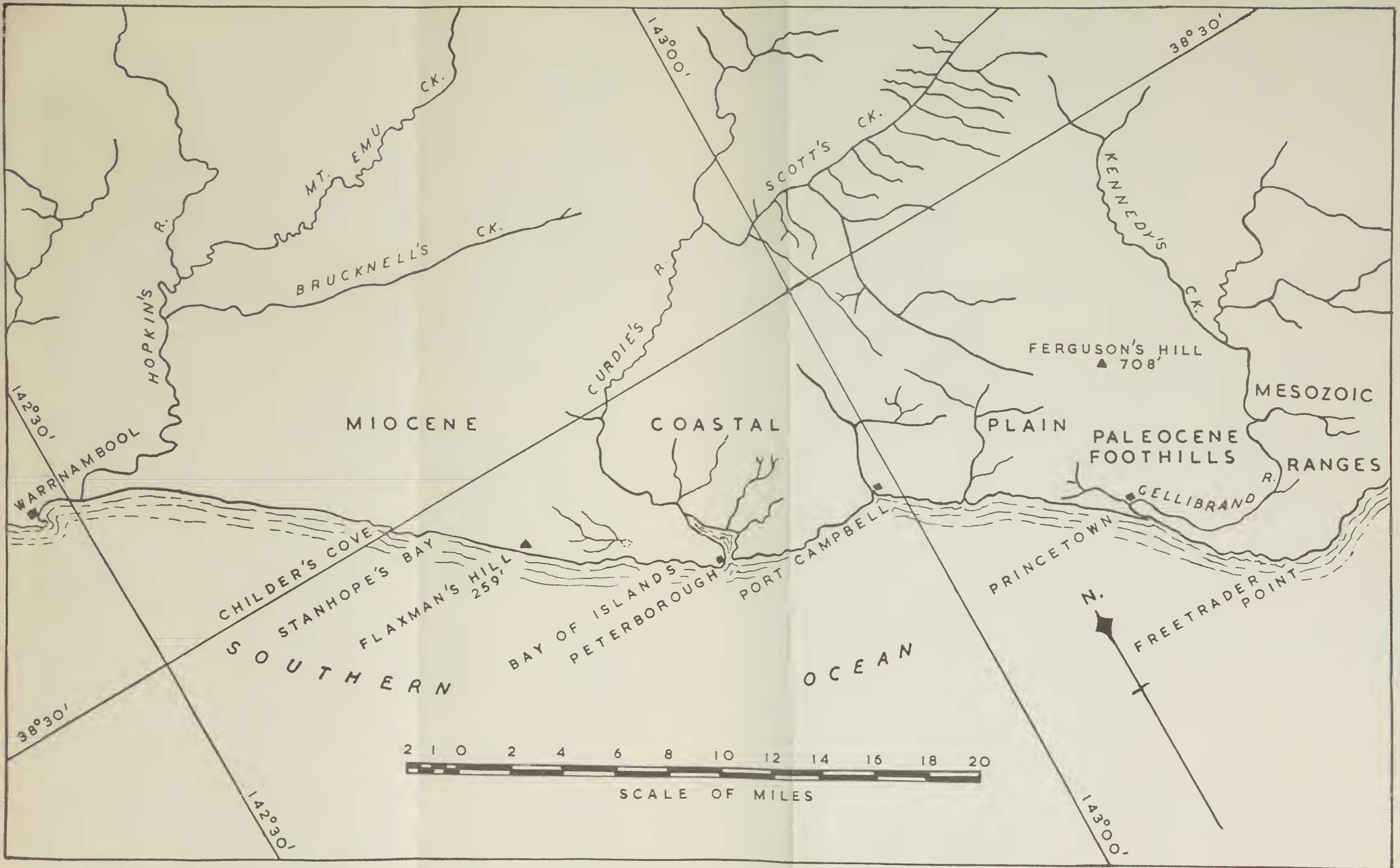
FIGURE 1.—Locality map of the coastal region between Freetrader Point and Warrnambool, South-western Victoria.
